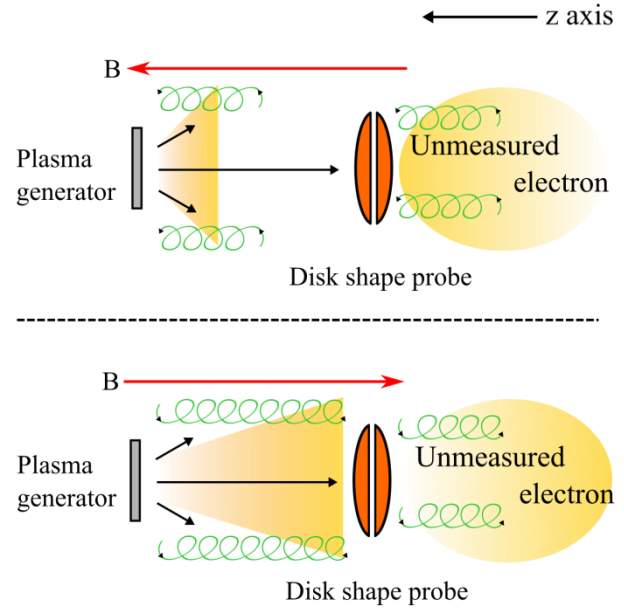
Figure 9 Effect of the magnetic field in the disk probe
