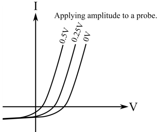
Figure 2 Principle of ETP probe
