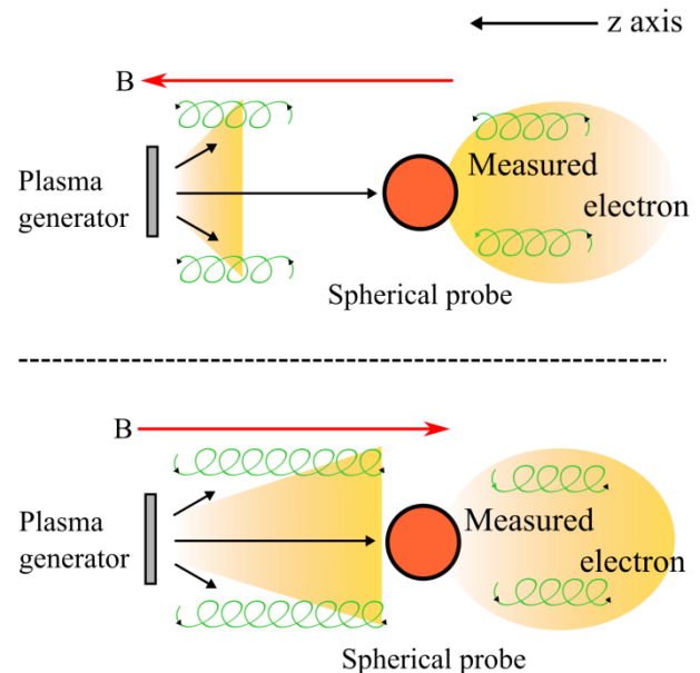
Figure 10 Effect of the magnetic field in the spherical probe
