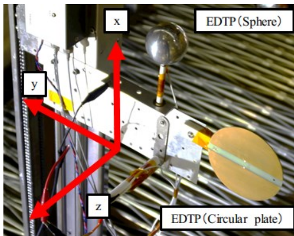
Figure 7 Each probe and magnetic field direction in the chamber
