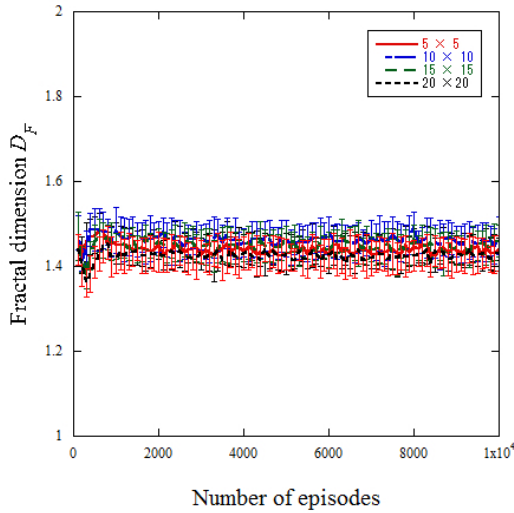
Figure 11 Result of non-learner with four grid world sizes
