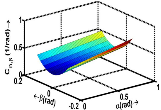
Figure 10 C_{n,\beta} at null rudder deflection
