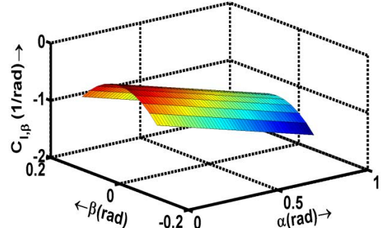
Figure 11 C_{l,\beta} at velocity 8 \text{ m}\cdot\text{s}^{-1}
