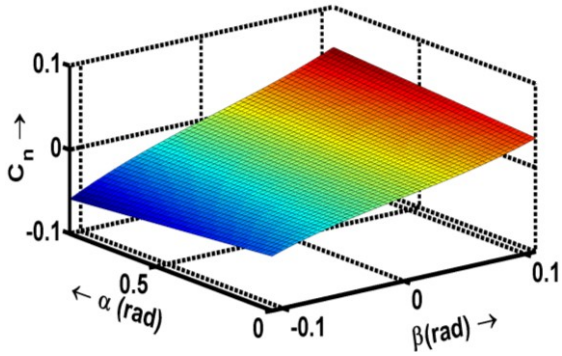
Figure 7 C_n at null rudder deflection
